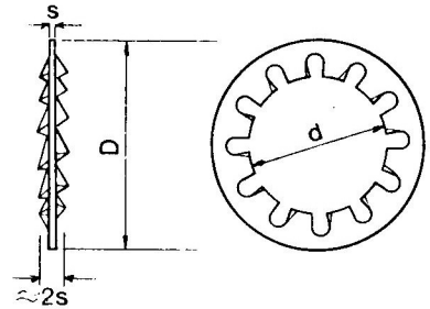
Type J (internal teeth)
