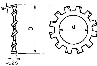
Type A (external teeth)
